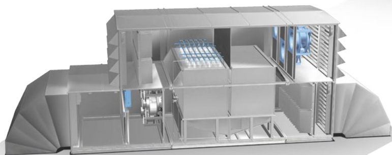
Adia-DENCO® Indirect Evaporative Cooling unit
