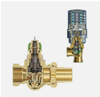
Pt40 & Rt40 Radiator Valve Sets
